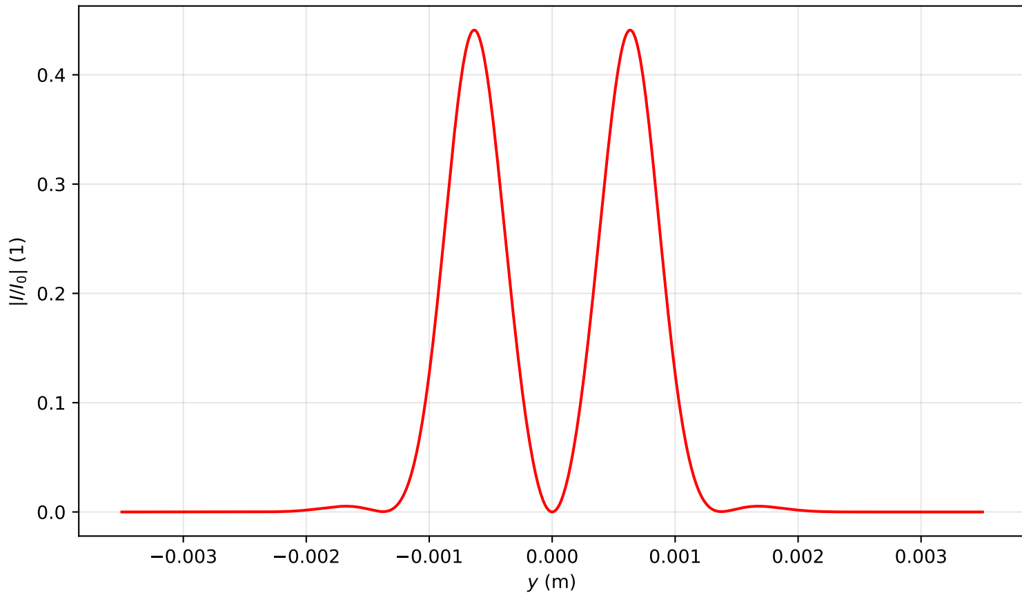
Intensity profile I(x=0, y, z=1.513)/I_0 , P_{in}=4.0P_{cr} , artificial time
